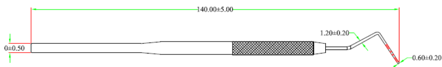
Front View
